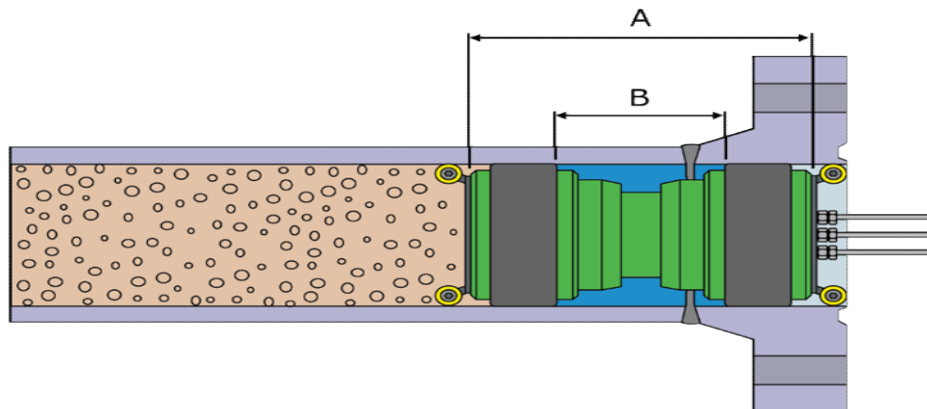
Hydraulic In-Line Weld Test Tool 3" up to 36"
